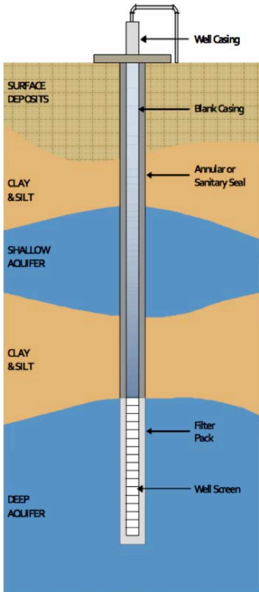
Figure 5. An example of typical well construction.
